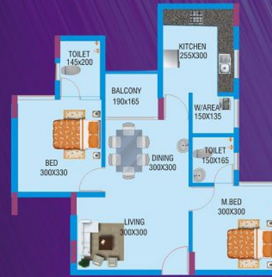
TYPE - J 2 BHK (2 to 8 th FLOOR) 1000 SQFT
